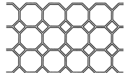
10" Octagon Tile Tile Size 262 x 262mm, Diamond Size 100 x 100mm
