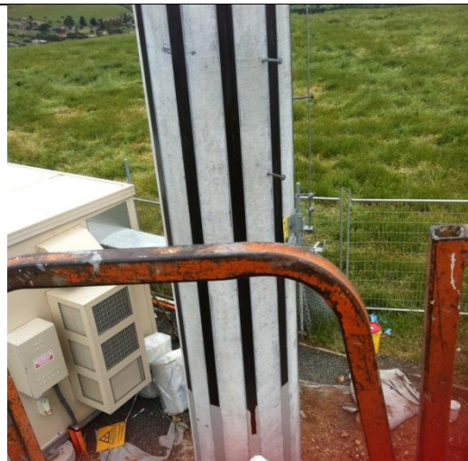
Monopole strengthening- Carbon laid in place before overcoating with UV membrane
